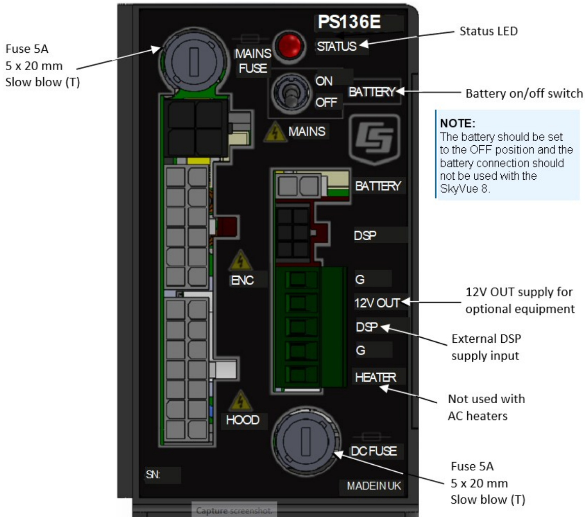
Figure 2-3. PSU types
