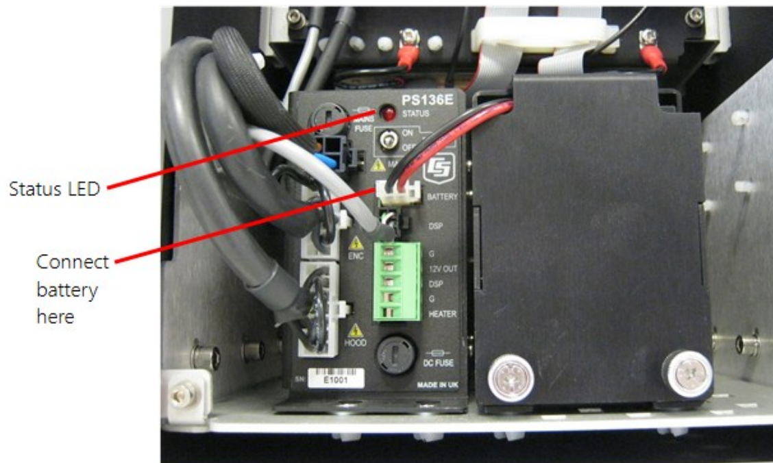
Figure 4-6. Connecting battery
